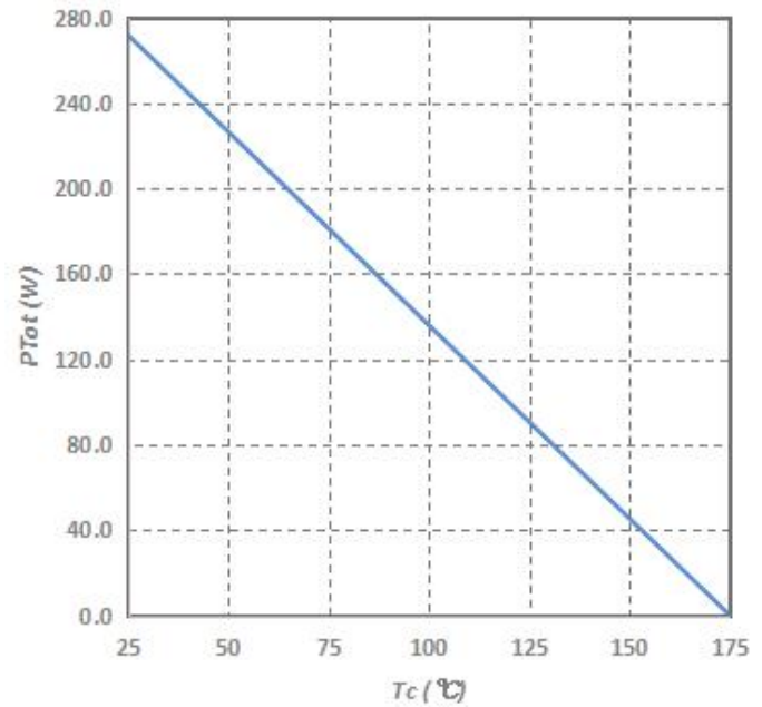
Fig.6-Power Derating
